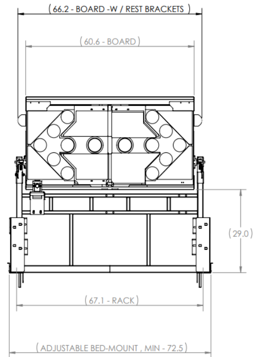
Assembled Dimmensions
